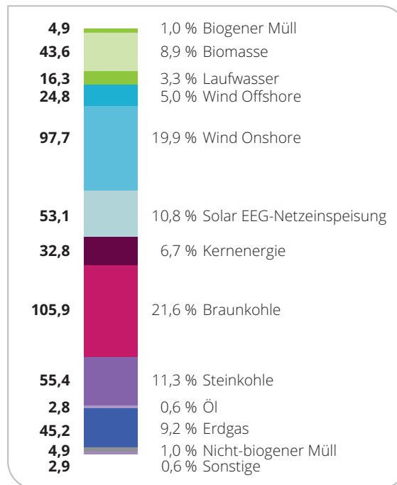
Abb. 92, Quelle: https://www.energy-charts.info/charts/energy_pie/chart.html?de&c=DE&interval=year&year=2022
